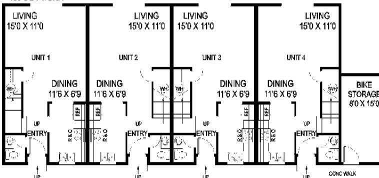
FIRST FLOOR PLAN 480 SQ FT/UNIT
