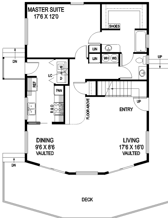
FIRST FLOOR PLAN 1059 SQ FT
