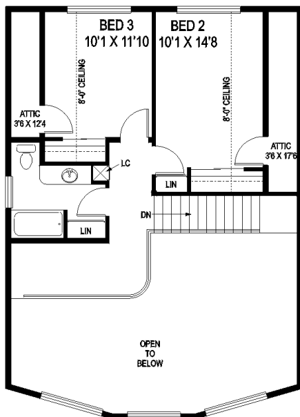
SECOND FLOOR PLAN 535 SQ FT
