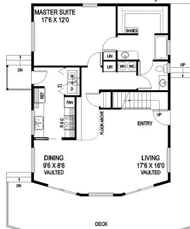
FIRST FLOOR PLAN 1059 SQ FT
