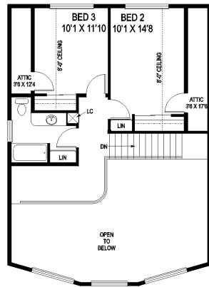
SECOND FLOOR PLAN 535 SQ FT
