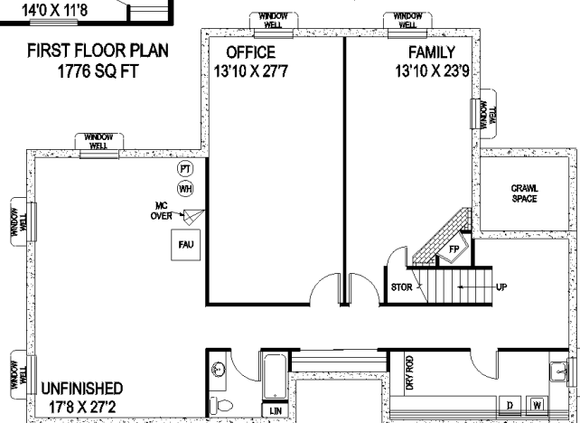
BASEMENT FLOOR PLAN 1826 SQ FT
